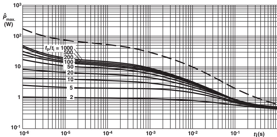
SFR16S Pulse on a regular basis; maximum permissible peak pulse power (Pmax-hat) as a function of pulse duration (ti)
