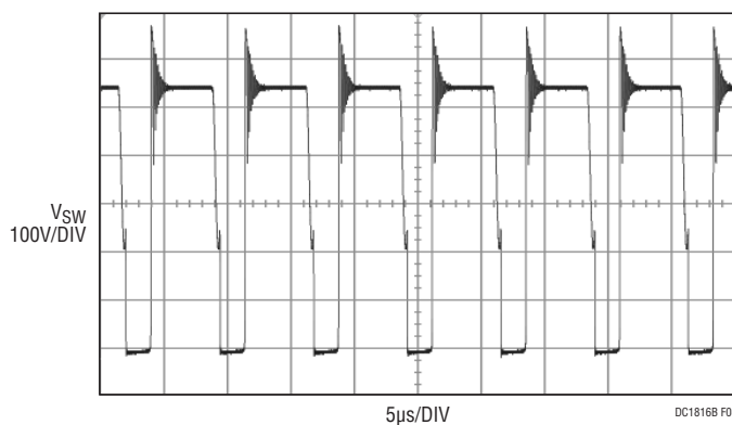
Figure 8. V_{IN} = 277VAC
