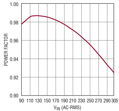
Figure 4. Power Factor vs Input Voltage
