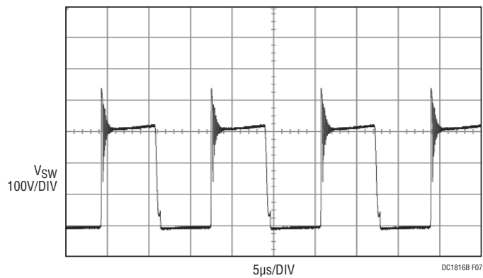
Figure 7. V_{IN} = 120VAC
