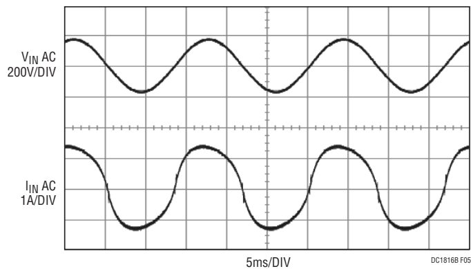
Figure 5. V_{IN} = 120VAC
