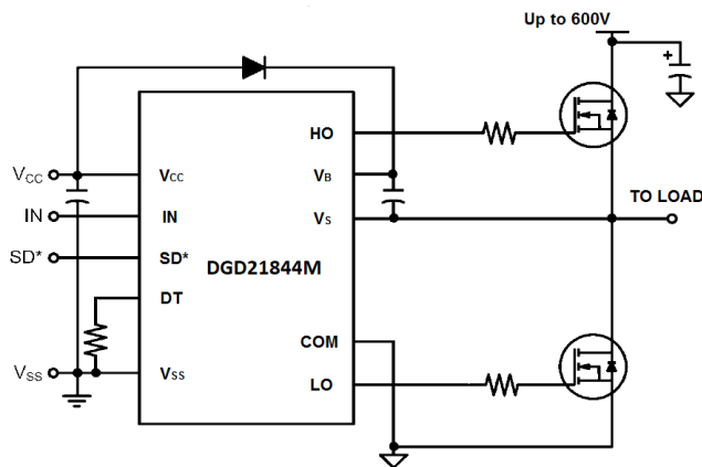
Typical Configuration
