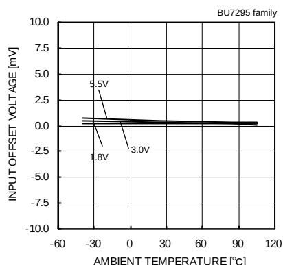
Fig.83 Input Offset Voltage – Ambient Temperature ( V_{icm}=V_{DD} , V_{OUT}=1.5[V] )
