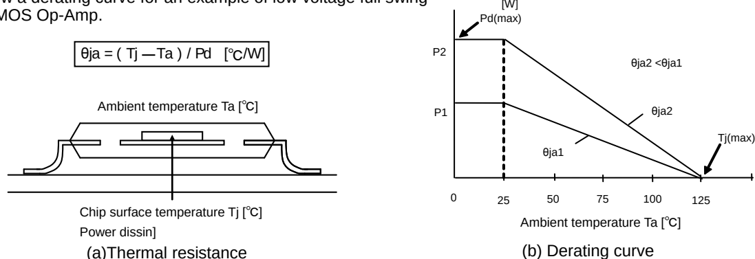
Fig. 195 Thermal resistance and derating
