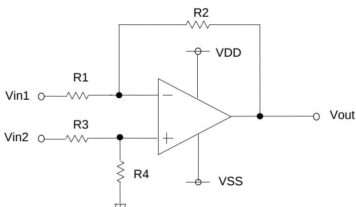
Fig. 194 Differential amplifier
