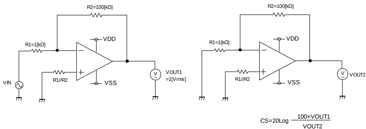
Fig.188 Test circuit 3
