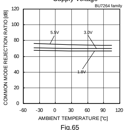
Fig. 65 Common Mode Rejection Ratio – Ambient Temperature
