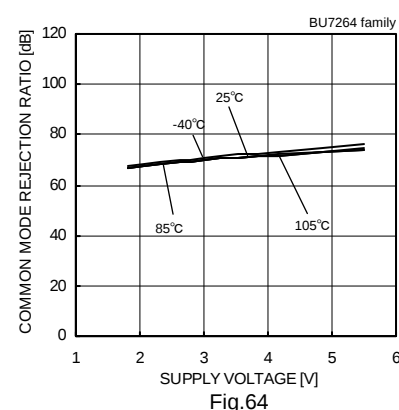
Fig. 64 Common Mode Rejection Ratio – Supply Voltage
