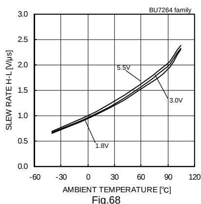
Fig. 68 Slew Rate H-L – Ambient Temperature
