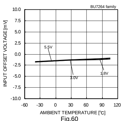
Fig. 60 Input Offset Voltage – Ambient Temperature ( V_{cm}=V_{DD} , V_{OUT}=1.5[V] )
