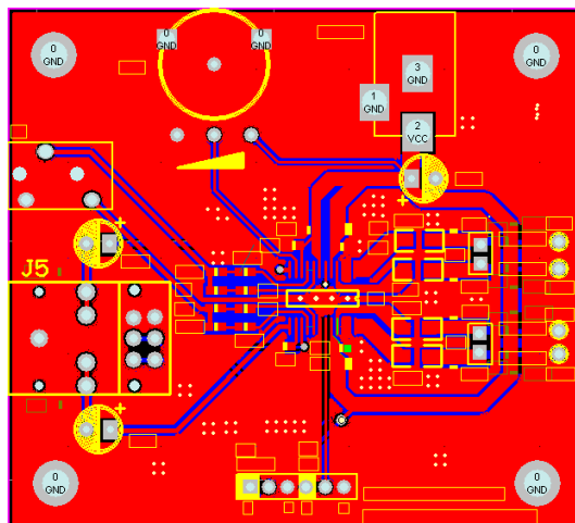
Figure 2: Top Layer
