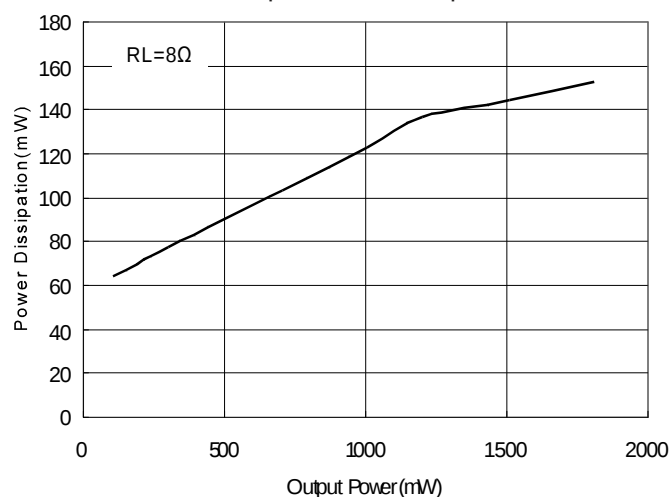
10. Power Dissipation vs Output Power
