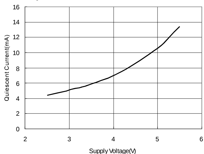
16. Quiescent Current
