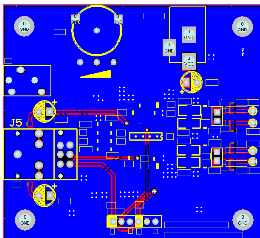
Figure 3: Bottom Layer
