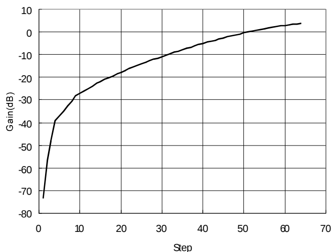
9. Gain Step
