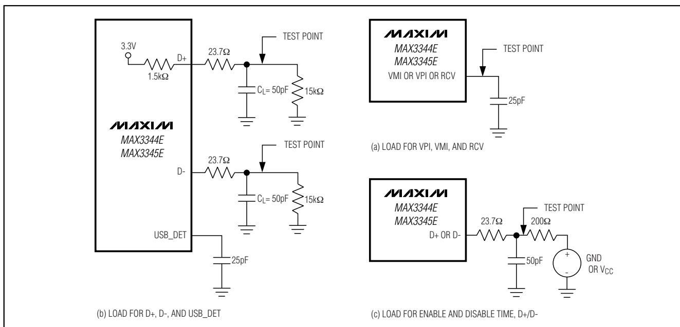
Figure 6. Test Circuits
