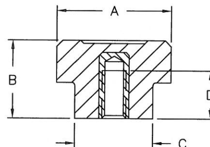
THREADED INTERNAL INSERT
