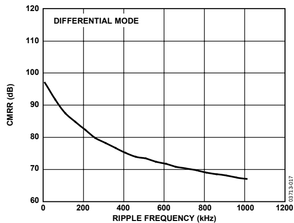
Figure 13. CMRR vs. Common-Mode Ripple with V_{DD} = 5\text{ V} and 3\text{ V}
