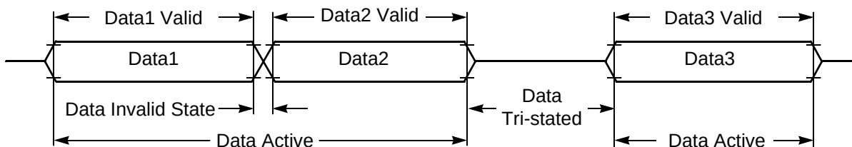
Figure 10-2 Signal States
