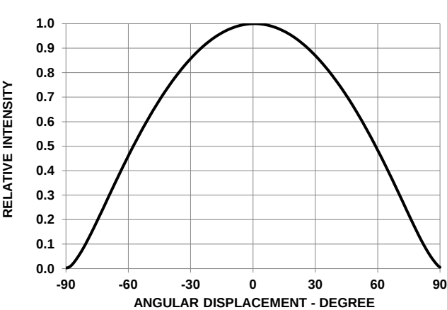
Figure 5: Radiation Pattern
