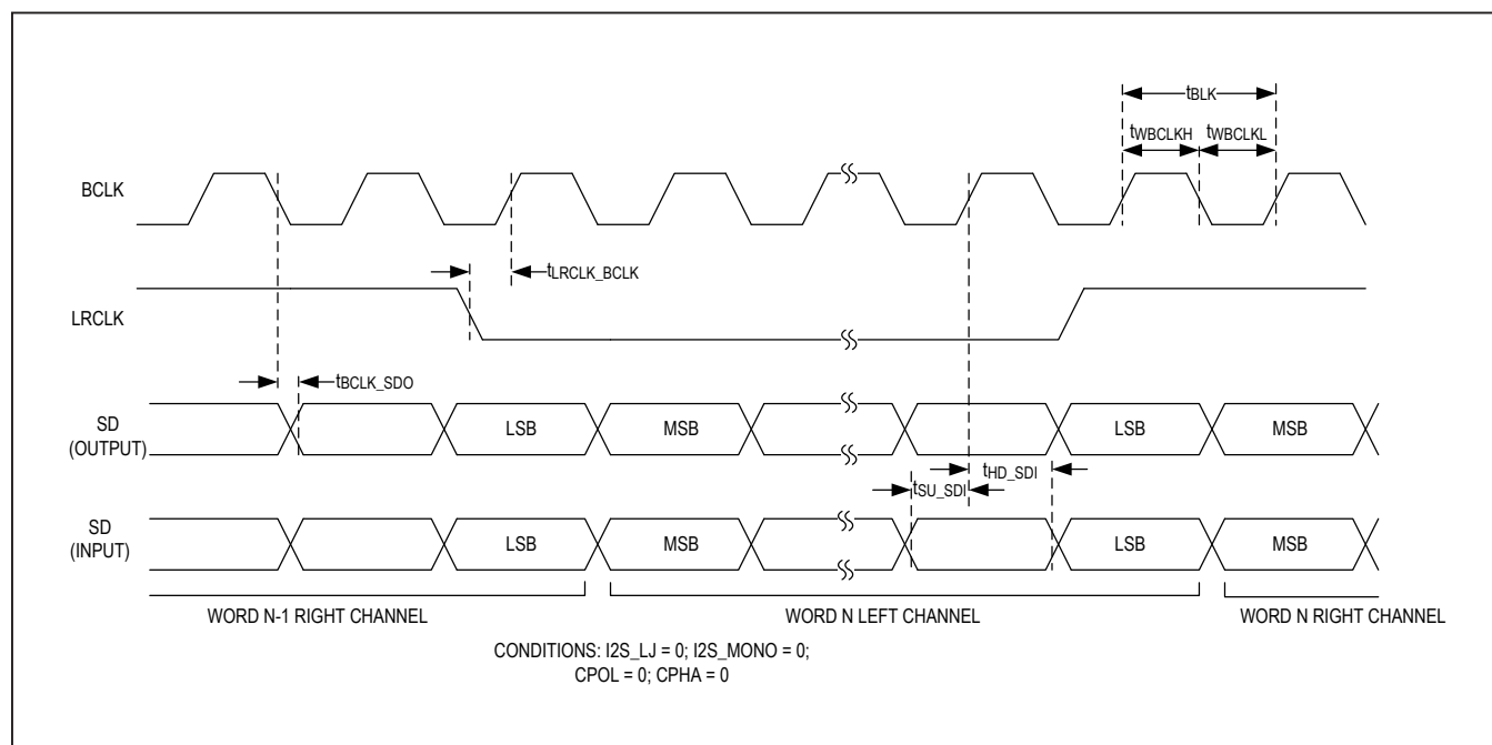
Figure 4. I 2 S Timing Diagram
