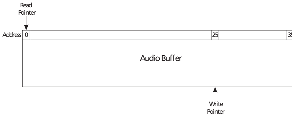
Figure 4-48: Audio Buffer After Initial 26 Sample Write
