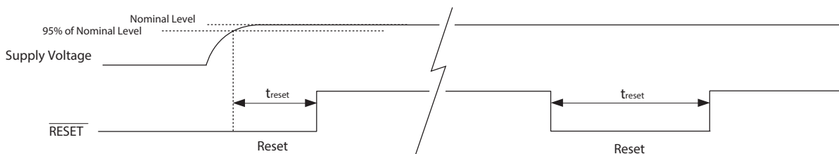
Figure 4-3: Reset Pulse
