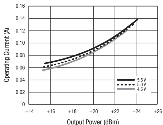
Figure 33. Operating Current vs Output Power Over VCC
