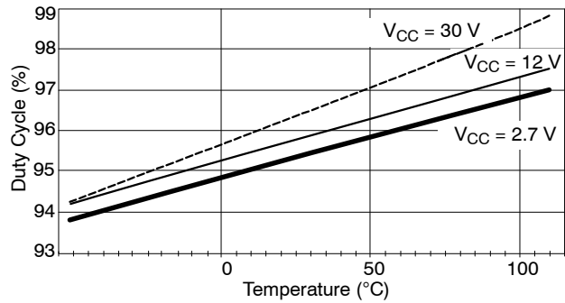
Figure 13. Maximum Duty Cycle vs. Temperature
