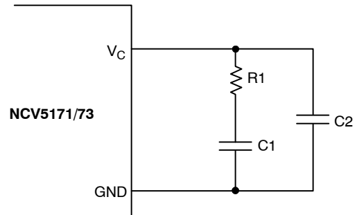
Figure 26. A Typical Compensation Network
