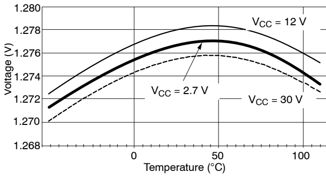
Figure 10. Reference Voltage vs. Temperature
