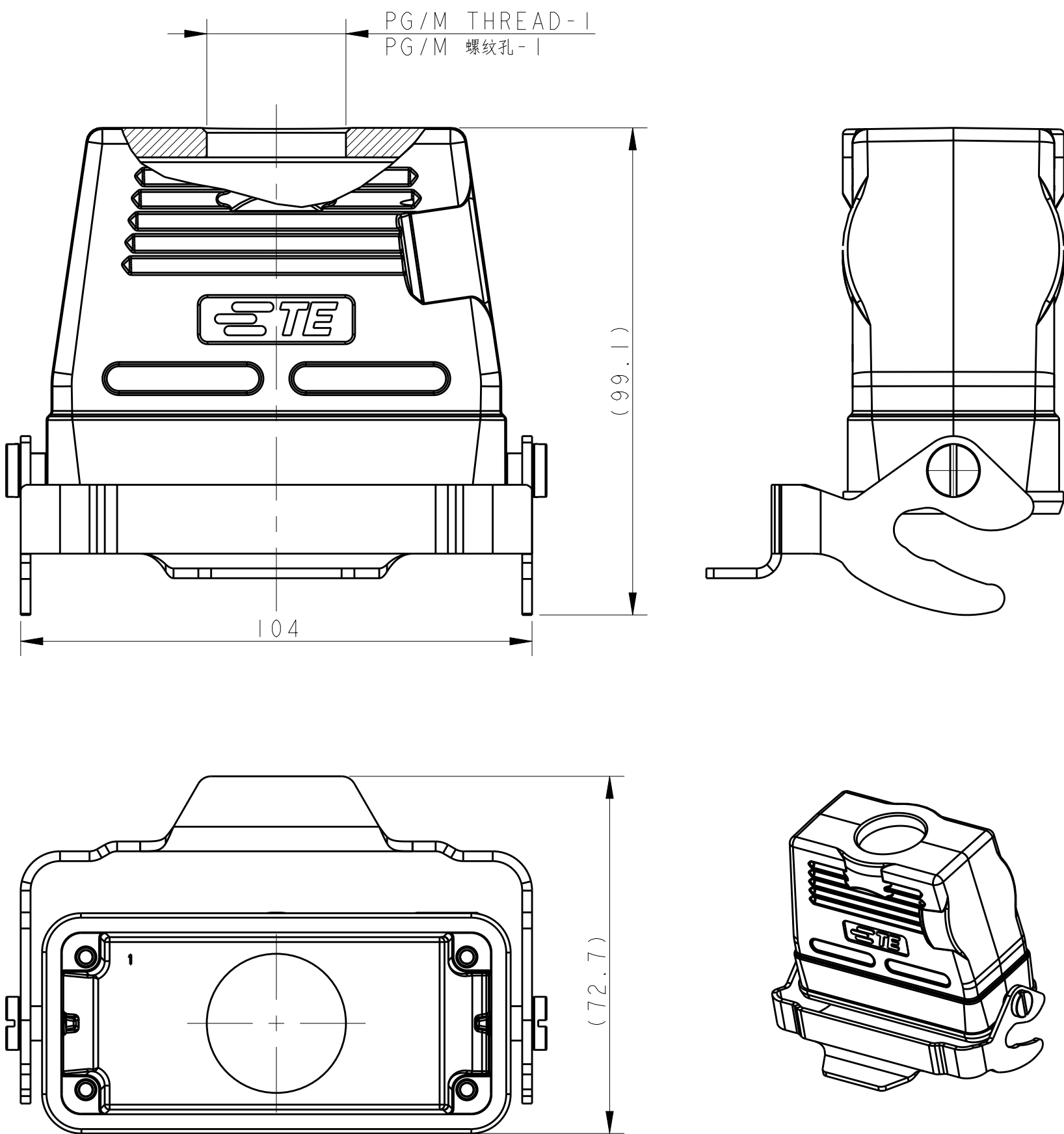
TYPE 9: HIGH CONSTRUCTION + METAL SINGLE LOCKING
