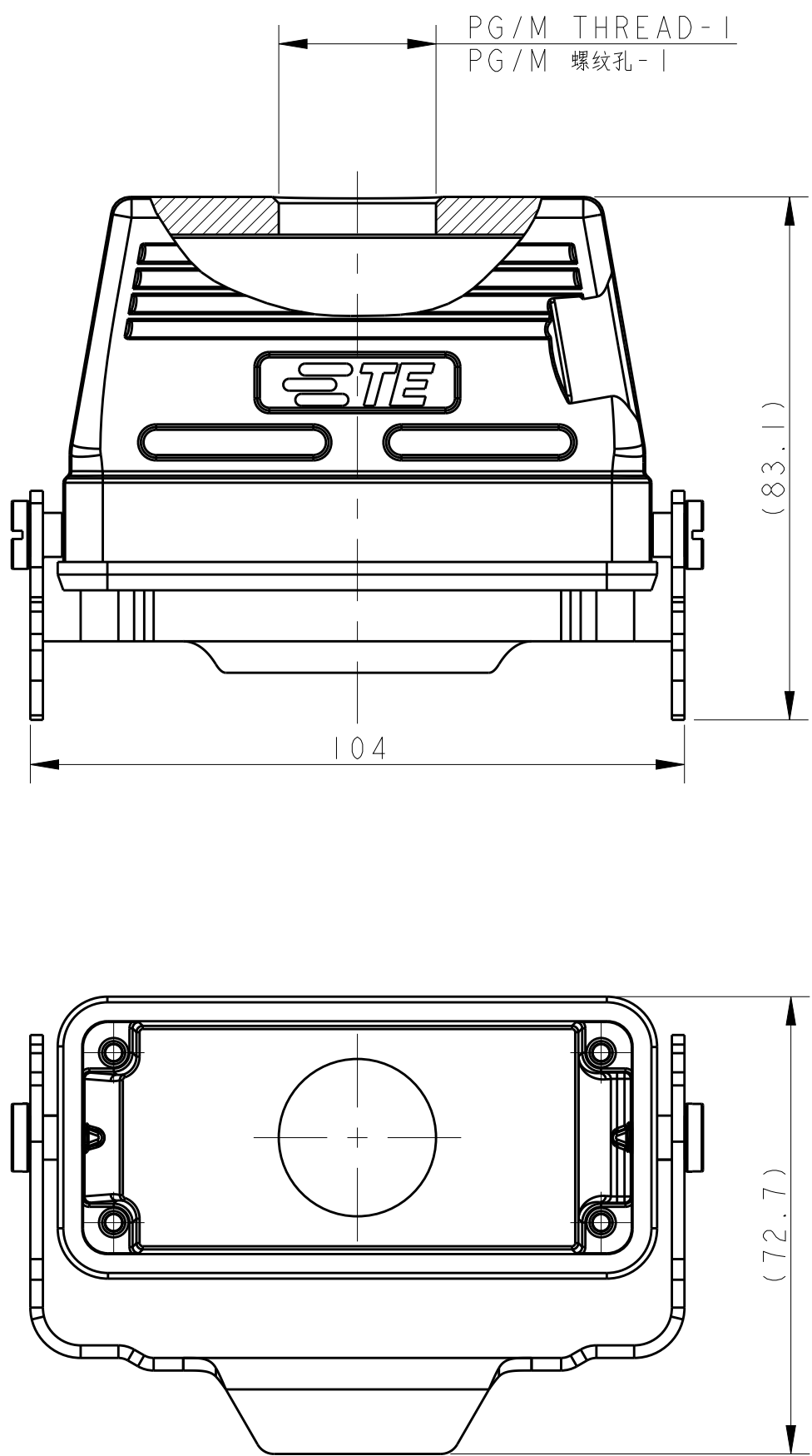
TYPE 4: LOW CONSTRUCTION + METAL SINGLE LOCKING OTHER SPEC REFER TO TYPE 1 类型4: 低结构壳体+彩锌单扣, 其他规格参照类型1
