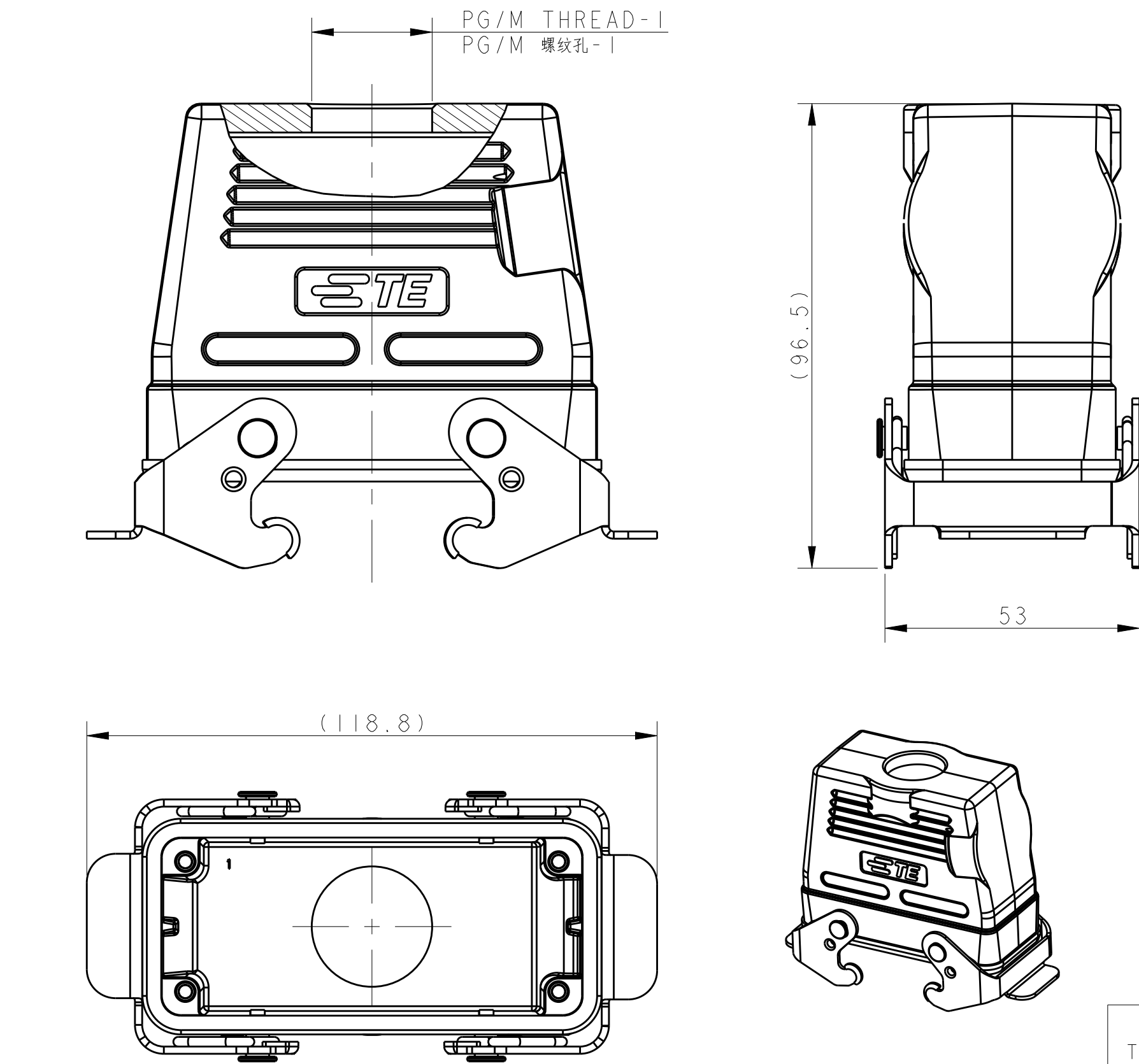
TYPE 6: HIGH CONSTRUCTION + METAL DOUBLE LOCKING
