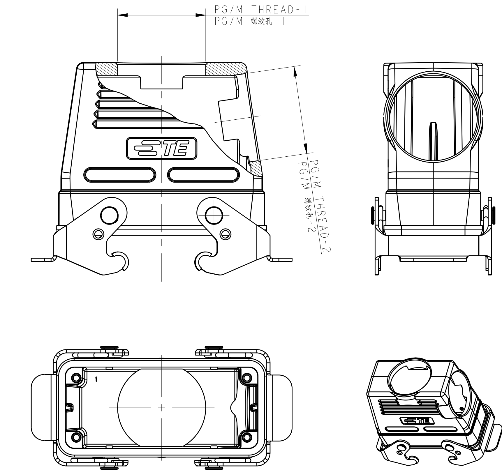
TYPE 8: HIGH CONSTRUCTION + METAL DOUBLE LOCKING
