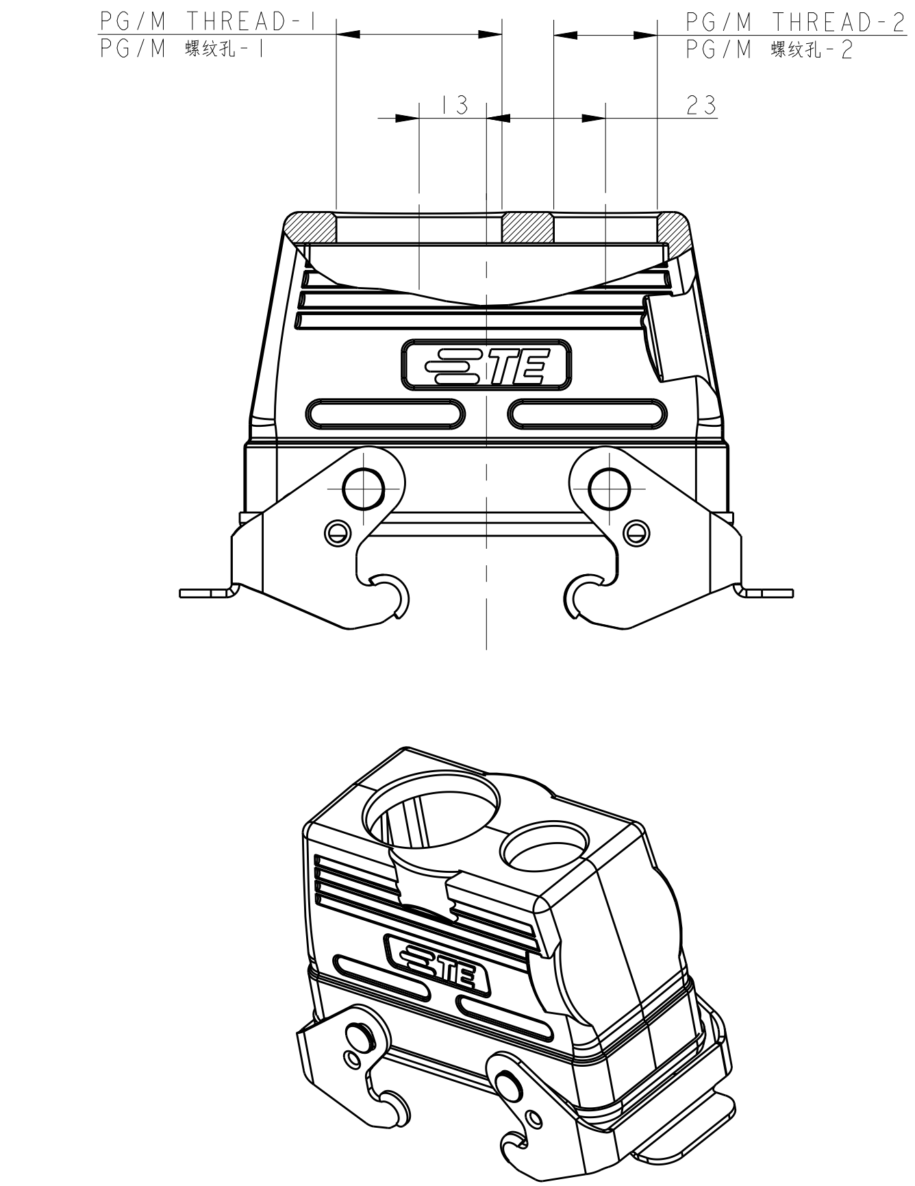
TYPE 3: LOW CONSTRUCTION + METAL DOUBLE LOCKING 2 ENTRY HOLE OTHER SPEC REFER TO TYPE 2 类型3: 低结构壳体+彩锌双扣, 2个进线孔, 其他规格参照类型2
