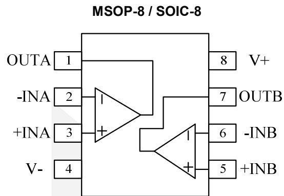
Figure 1 Top View
