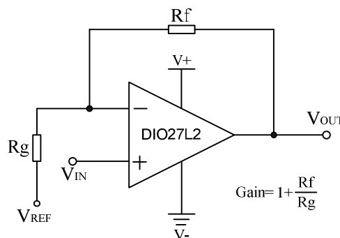
Non-Inverting Amplifier
