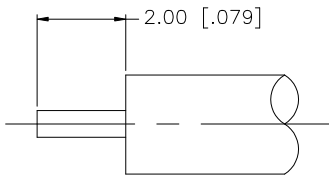
RECOMMENDED CABLE STRIPPING DIMENSIONS
