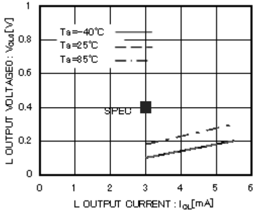
Figure 10. 'L' Output Voltage0 V_{OL0}-I_{OL}(V_{CC0}=3.0V)
