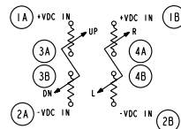
C. ISOLATED GAGES (8 TERMINALS)
