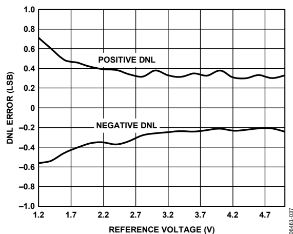
Figure 8. DNL Error vs. Reference Voltage, f_{SCL} = 1.7MHz Without Clock Stretching
