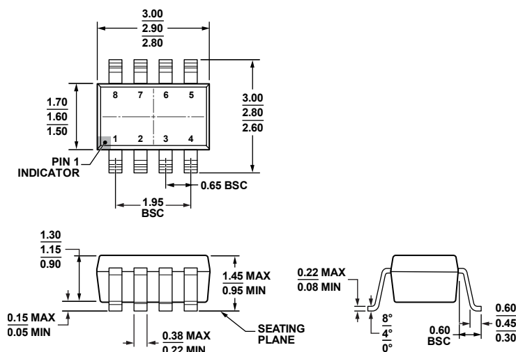
Figure 29. 8-Lead Small Outline Transistor Package [SOT-23]
