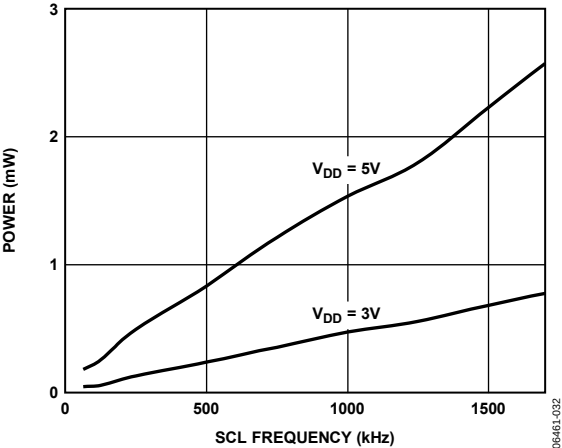
Figure 17. Power vs. SCL Frequency, V_{REF} = 2.5\text{ V}
