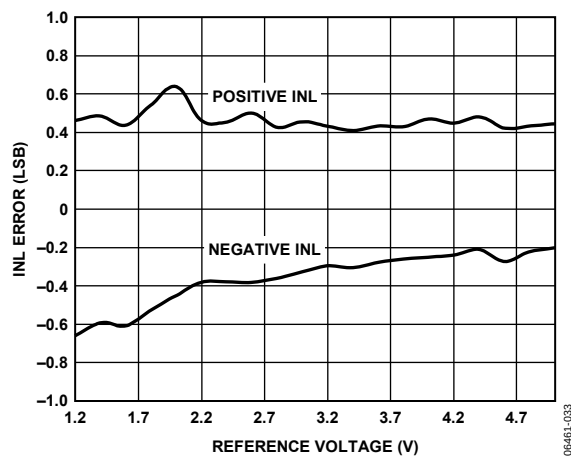
Figure 7. INL Error vs. Reference Voltage, f_{SCL} = 1.7MHz Without Clock Stretching
