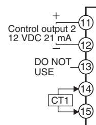
E53-CNQH2 Control Output 2 and CT
