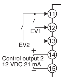
E53-CNQB2 Event Inputs and Control Output 2
