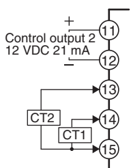
E53-CNQH2 Control Output 2 and CT2
