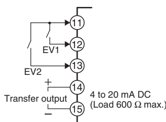
E53-CNBF2 Event Inputs and Transfer Output
