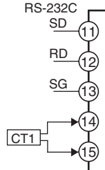
E53-CNH01N2 Communications (RS-232) and CT
