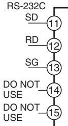
E53-CN01N2 Communications (RS-232)
