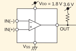
Figure 2: Voltage Application Allowed When V_{DD} = 0 V
