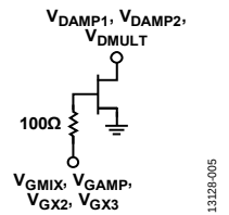
Figure 5. V_{DAMP1} , V_{DAMP2} , V_{DMULT} , V_{GAMP} , V_{GMIX} , V_{GX2} , and V_{GX3} Interface
