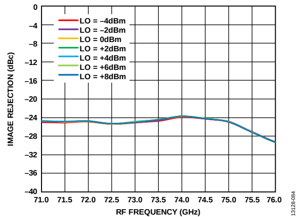
Figure 80. Image Rejection vs. RF Frequency at Various LO Powers, RFIN = -20 dBm, IF = 2000 MHz, V_{DLNA} = 3 V
