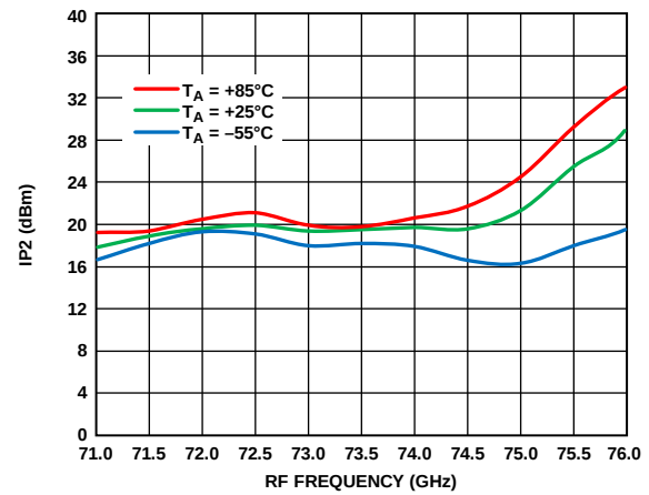
Figure 30. Input IP2 vs. RF Frequency at Various Temperatures, R_{FIN} = -20\text{ dBm} , LO = 2\text{ dBm} , IF = 1000\text{ MHz} , V_{DLNA} = 3\text{ V}
