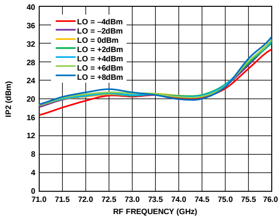
Figure 28. Input IP2 vs. RF Frequency at Various LO Powers, R_{FIN} = -20\text{ dBm} , IF = 1000\text{ MHz} , V_{DLNA} = 4\text{ V}
