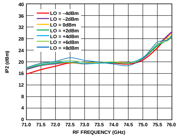
Figure 31. Input IP2 vs. RF Frequency at Various LO Powers, R_{FIN} = -20\text{ dBm} , IF = 1000\text{ MHz} , V_{DLNA} = 3\text{ V}
