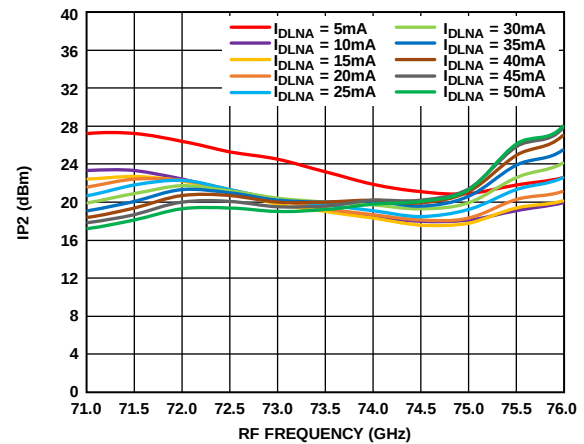
Figure 32. Input IP2 vs. RF Frequency at Various I_{DLNA} Values, R_{FIN} = -20\text{ dBm} , LO = 2\text{ dBm} , IF = 1000\text{ MHz} , V_{DLNA} = 3\text{ V}
