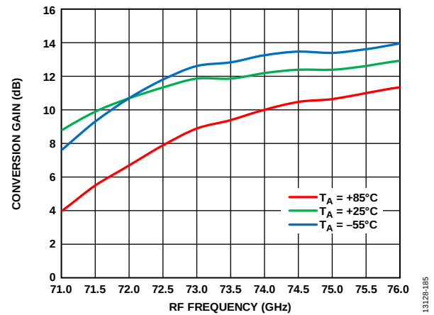
Figure 169. Conversion Gain vs. RF Frequency at Various Temperatures, RFIN = -20 dBm, LO = 2 dBm, IF = 2000 MHz, V_{DLN} = 3 V
