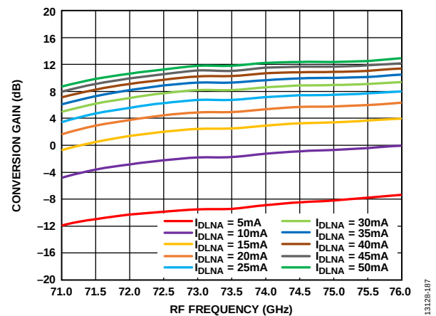
Figure 171. Conversion Gain vs. RF Frequency at Various I_{DLN} Values, RFIN = -20 dBm, IF = 2000 MHz, V_{DLN} = 3 V
