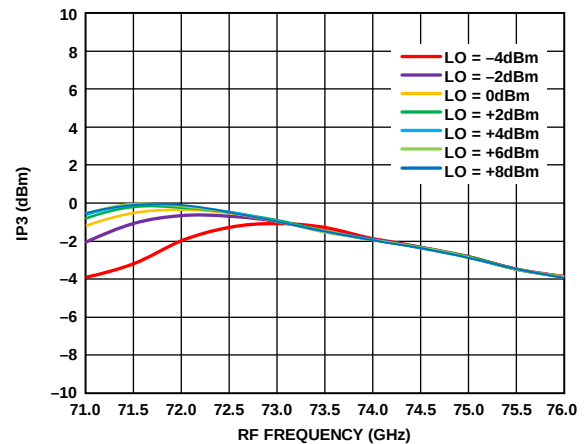
Figure 60. Input IP3 vs. RF Frequency at Various LO Powers, RFIN = -20 dBm, IF = 500 MHz, V_{DLNA} = 3 V
