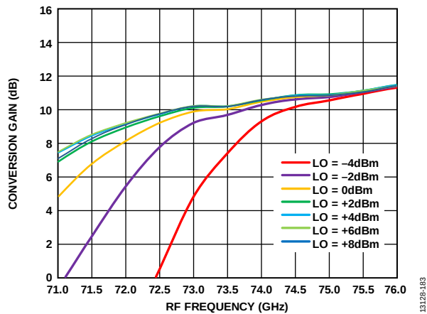
Figure 167. Conversion Gain vs. RF Frequency at Various LO Powers, RFIN = -20 dBm, IF = 2000 MHz, V_{DLN} = 4 V
