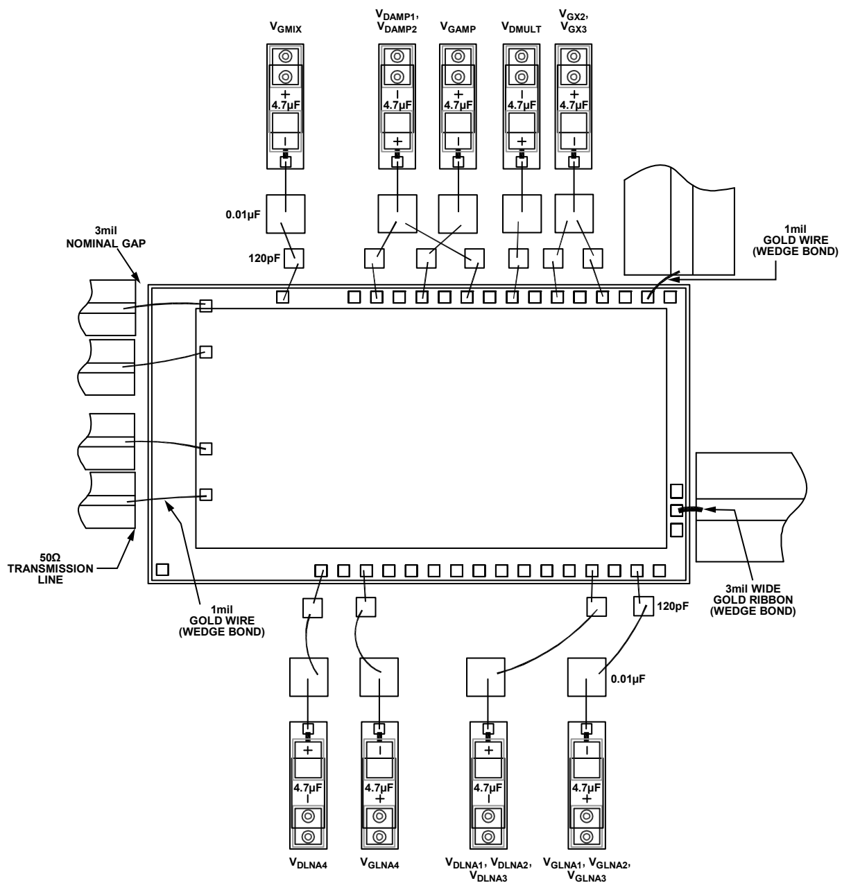
Figure 213. Assembly Diagram
