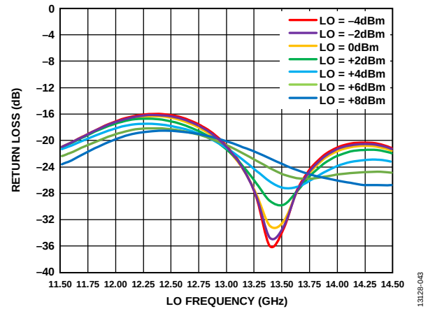
Figure 43. LO Return Loss vs. LO Frequency at Various LO Powers, V_{DLNA} = 4 V
