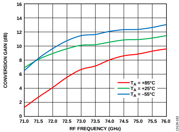
Figure 166. Conversion Gain vs. RF Frequency at Various Temperatures, RFIN = -20 dBm, LO = 2 dBm, IF = 2000 MHz, V_{DLN} = 4 V
