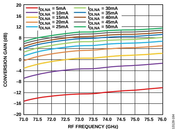
Figure 168. Conversion Gain vs. RF Frequency at Various I_{DLN} Values, RFIN = -20 dBm, IF = 2000 MHz, V_{DLN} = 4 V
