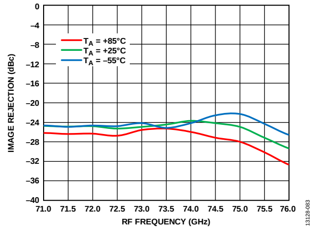
Figure 79. Image Rejection vs. RF Frequency at Various Temperatures, RFIN = -20 dBm, LO = 2 dBm, IF = 2000 MHz, V_{DLNA} = 3 V
