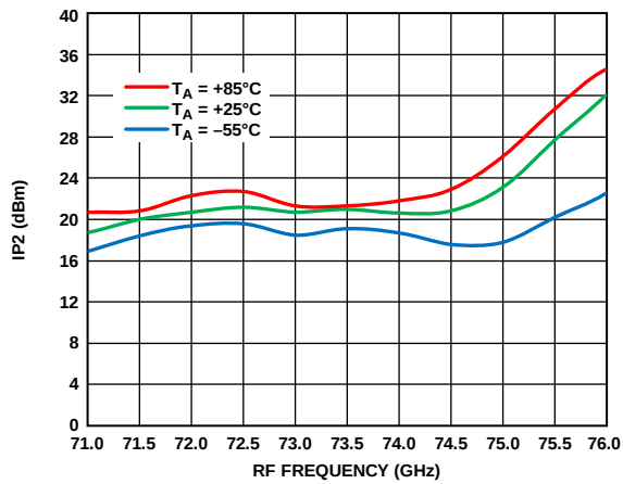
Figure 27. Input IP2 vs. RF Frequency at Various Temperatures, R_{FIN} = -20\text{ dBm} , LO = 2\text{ dBm} , IF = 1000\text{ MHz} , V_{DLNA} = 4\text{ V}
