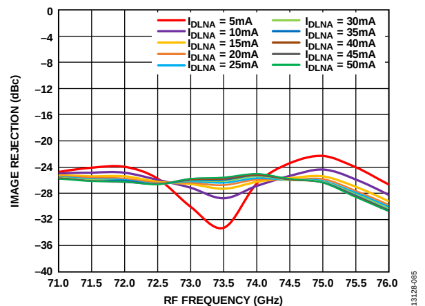
Figure 81. Image Rejection vs. RF Frequency at Various I_{DLNA} Values, RFIN = -20 dBm, LO = 2 dBm, IF = 2000 MHz, V_{DLNA} = 3 V
