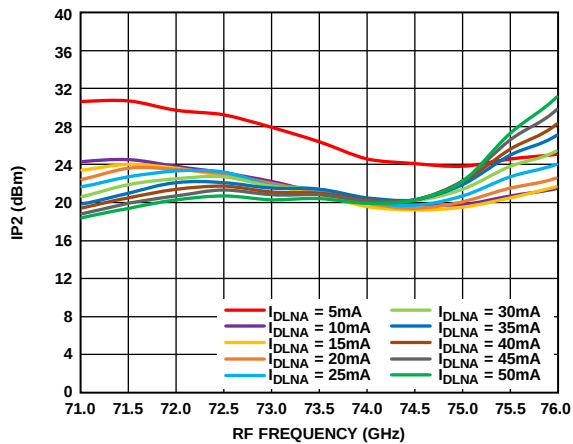
Figure 29. Input IP2 vs. RF Frequency at Various I_{DLNA} Values, R_{FIN} = -20\text{ dBm} , LO = 2\text{ dBm} , IF = 1000\text{ MHz} , V_{DLNA} = 4\text{ V}
