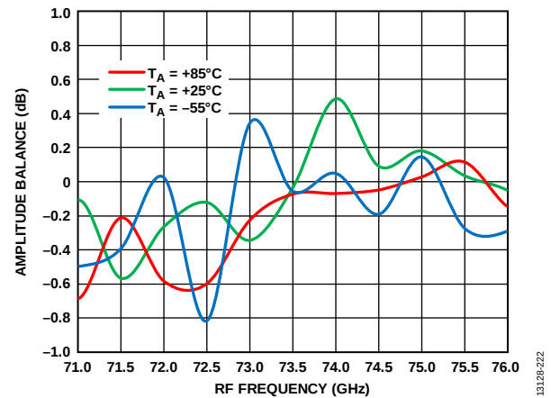
Figure 202. Amplitude Balance vs. RF Frequency at Various Temperatures, RFIN = -20 dBm, LO = 2 dBm, IF = 1000 MHz, V_{DLNA} = 3 V
