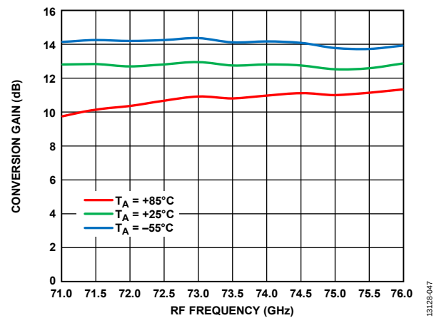
Figure 47. Conversion Gain vs. RF Frequency at Various Temperatures, R_{FIN} = -20 dBm, LO = 2 dBm, IF = 500 MHz, V_{DLNA} = 3 V
