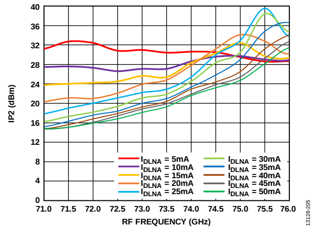
Figure 189. Input IP2 vs. RF Frequency at Various I_{DLNA} Values, R_{FIN} = -20 dBm, LO = 2 dBm, IF = 2000 MHz, V_{DLNA} = 3 V
