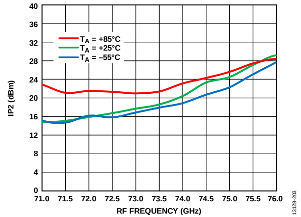
Figure 187. Input IP2 vs. RF Frequency at Various Temperatures, R_{FIN} = -20 dBm, LO = 2 dBm, IF = 2000 MHz, V_{DLNA} = 3 V
