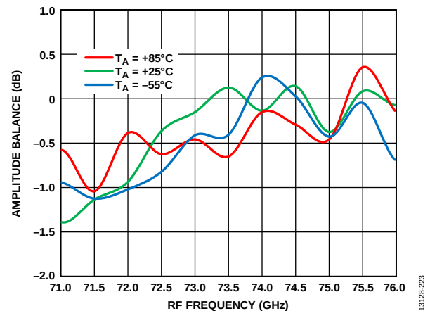
Figure 203. Amplitude Balance vs. RF Frequency at Various Temperatures, RFIN = -20 dBm, LO = 2 dBm, IF = 2000 MHz, V_{DLNA} = 3 V
