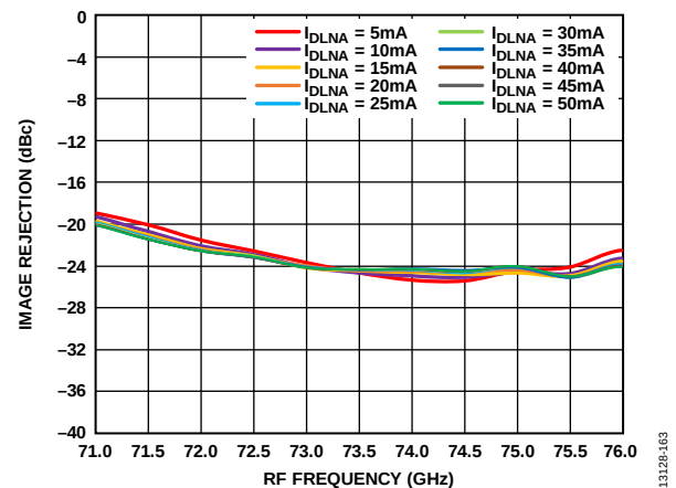
Figure 151. Image Rejection vs. RF Frequency at Various I_{DLNA} Values, RFIN = -20 dBm, LO = 2 dBm, IF = 1000 MHz, V_{DLNA} = 3 V
