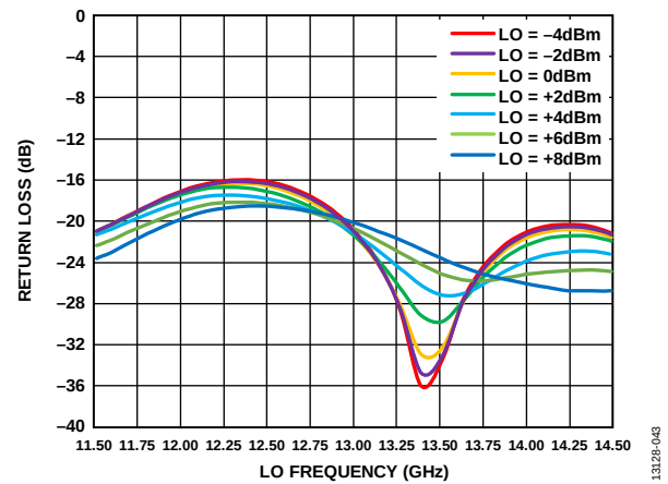
Figure 43. LO Return Loss vs. LO Frequency at Various LO Powers, V_{DLNA} = 4 \text{ V}
