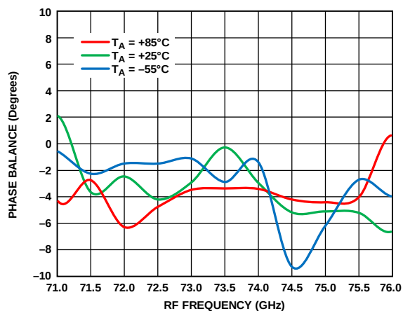
Figure 206. Phase Balance vs. RF Frequency at Various Temperatures, RFIN = -20 dBm, LO = 2 dBm, IF = 2000 MHz, V_{DLN} = 4 V
