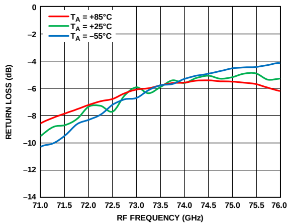
Figure 39. RF Return Loss vs. RF Frequency at Various Temperatures, LO = 2 \text{ dBm} , LO = 12 \text{ GHz} , V_{DLNA} = 4 \text{ V}
