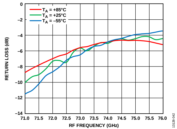
Figure 42. RF Return Loss vs. RF Frequency at Various Temperatures, LO = 2 \text{ dBm} , LO = 12 \text{ GHz} , V_{DLNA} = 3 \text{ V}
