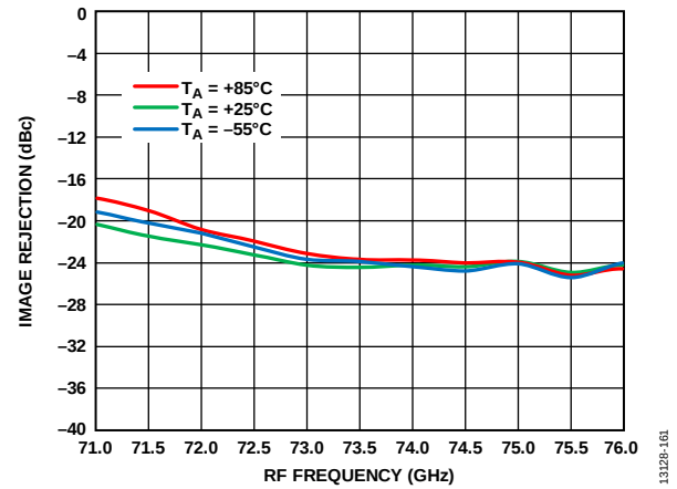
Figure 149. Image Rejection vs. RF Frequency at Various Temperatures, RFIN = -20 dBm, LO = 2 dBm, IF = 1000 MHz, V_{DLNA} = 3 V
