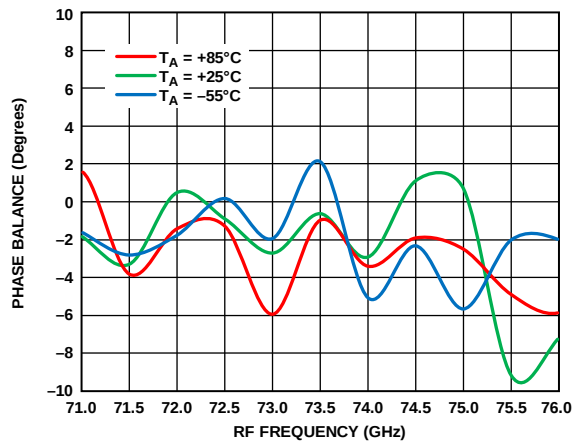
Figure 205. Phase Balance vs. RF Frequency at Various Temperatures, RFIN = -20 dBm, LO = 2 dBm, IF = 1000 MHz, V_{DLN} = 4 V
