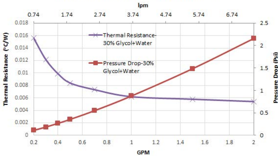
Thermal Resistance And Pressure Drop ATS-CP-1000
