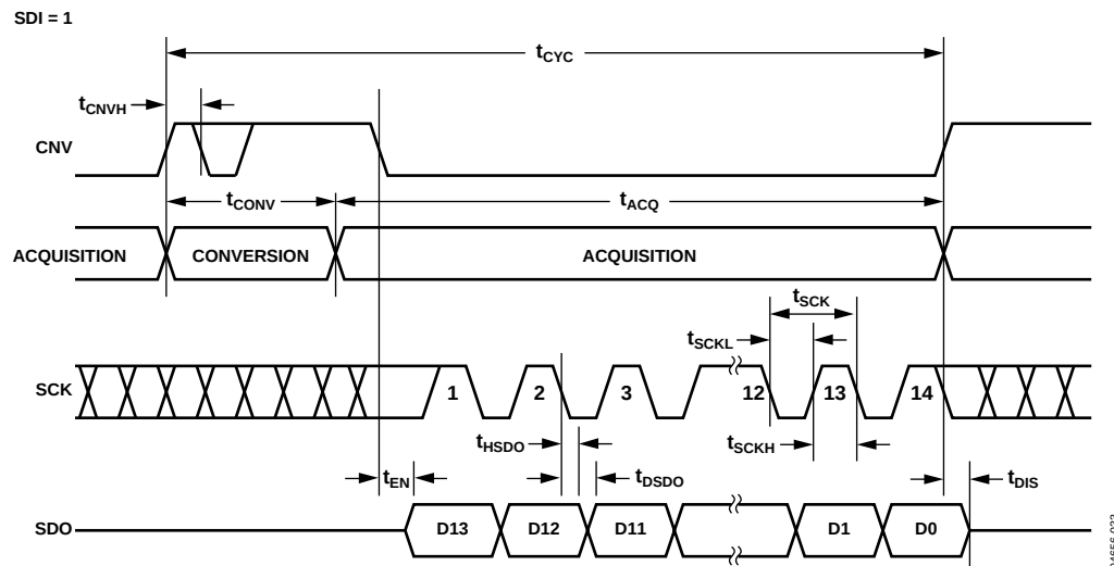
Figure 34. \overline{\text{CS}} Mode 3-Wire, No BUSY Indicator Serial Interface Timing (SDI High)
