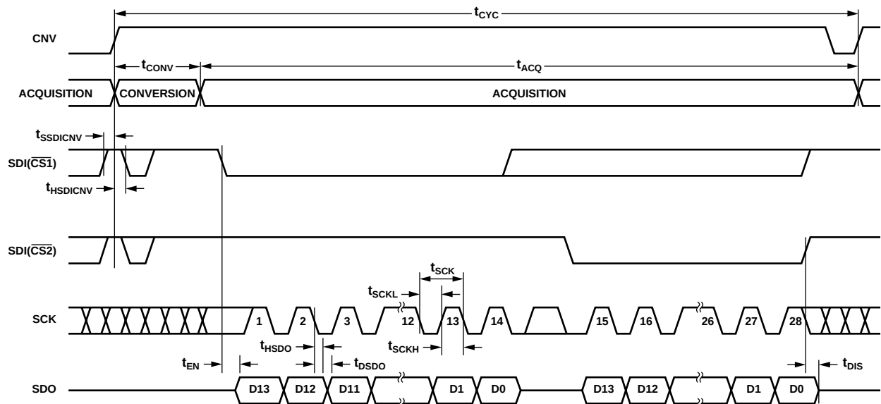
Figure 38. \overline{\text{CS}} Mode 4-Wire, No BUSY Indicator Serial Interface Timing
