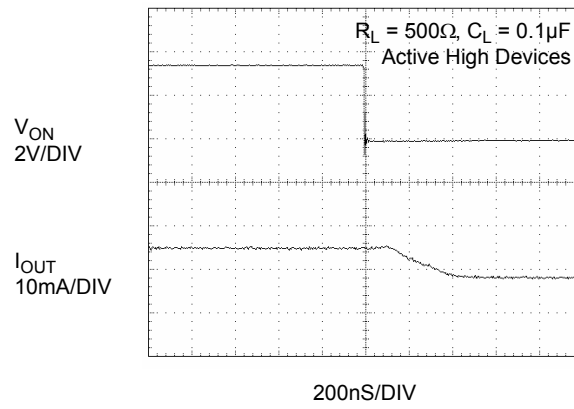
Figure 16. T OFF Response
