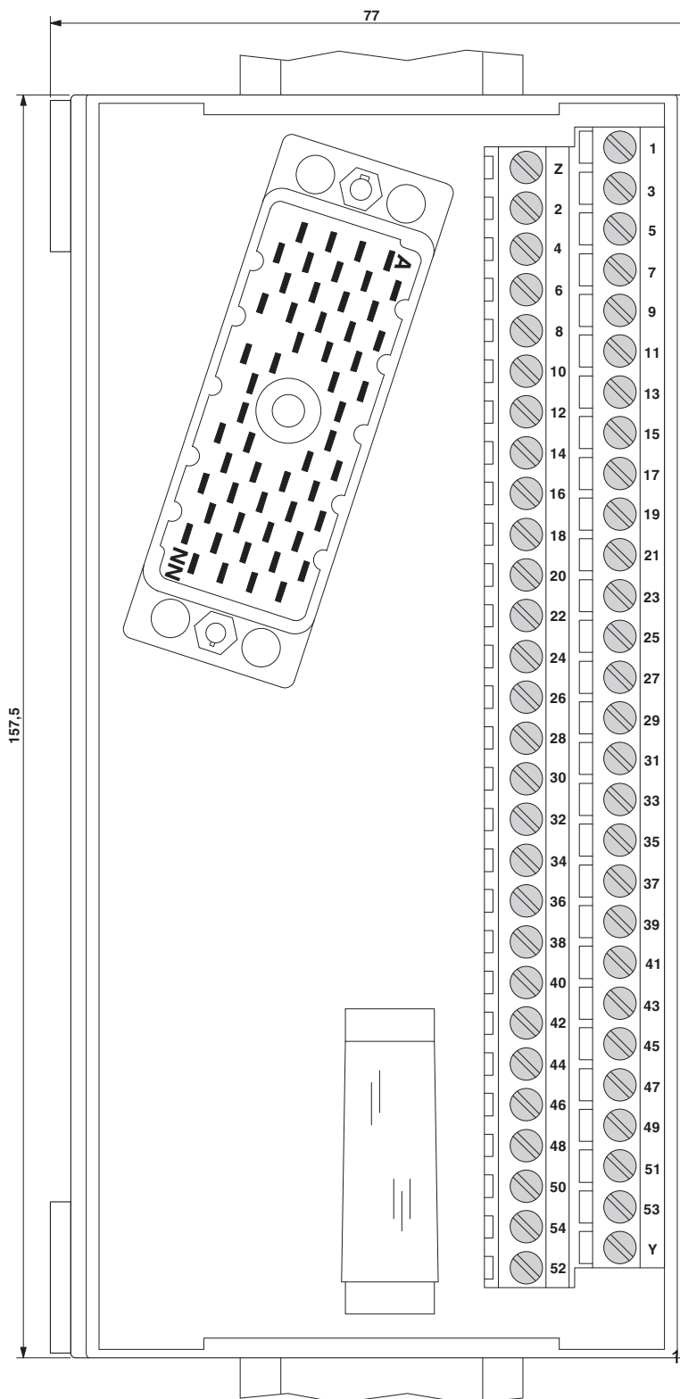
Dimensioned drawing
