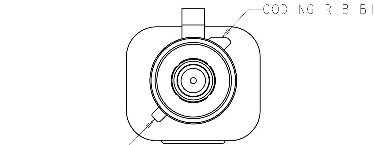
DETAIL G
