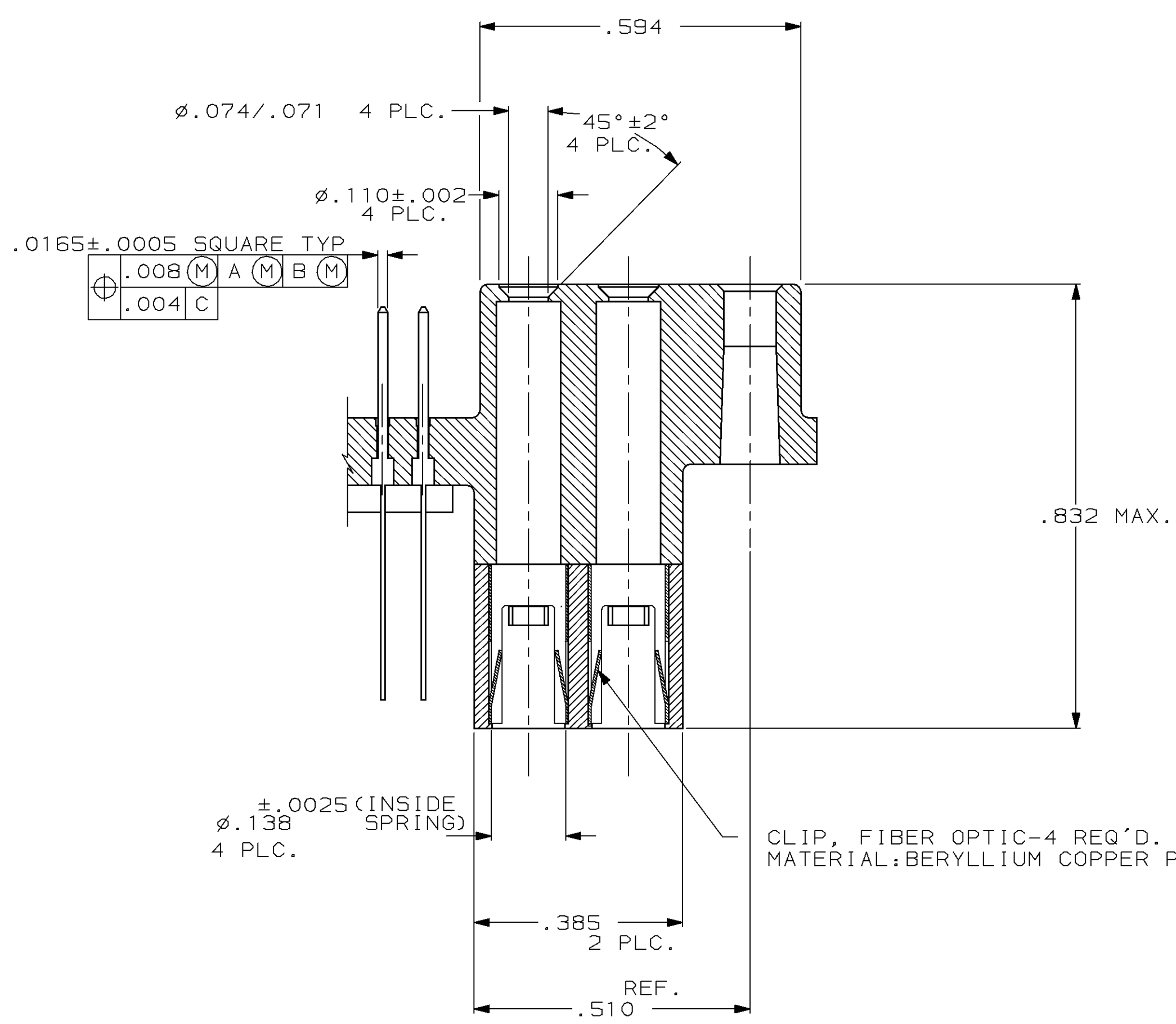
SECTION Y-Y SCALE 5:1
