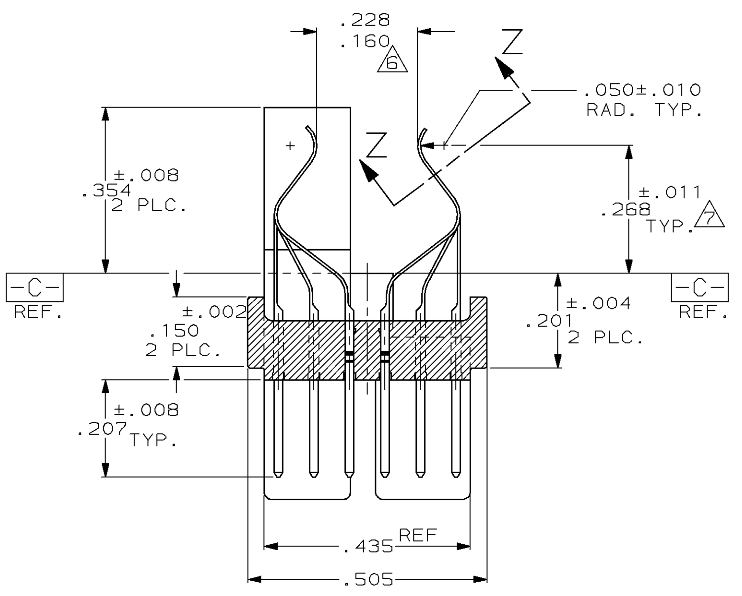
SECTION W-W SCALE 5:1 ROTATED CCW 90° (445269-1 ONLY)
