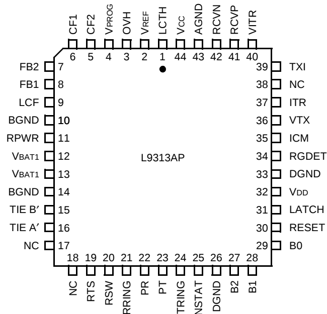
Figure 2. 44-Pin PLCC
