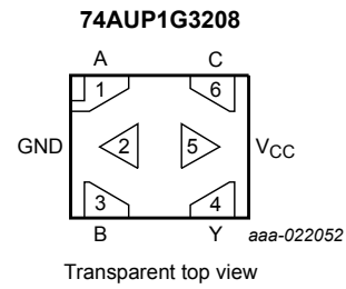
Figure 5. Pin configuration SOT1255 (X2SON6)
