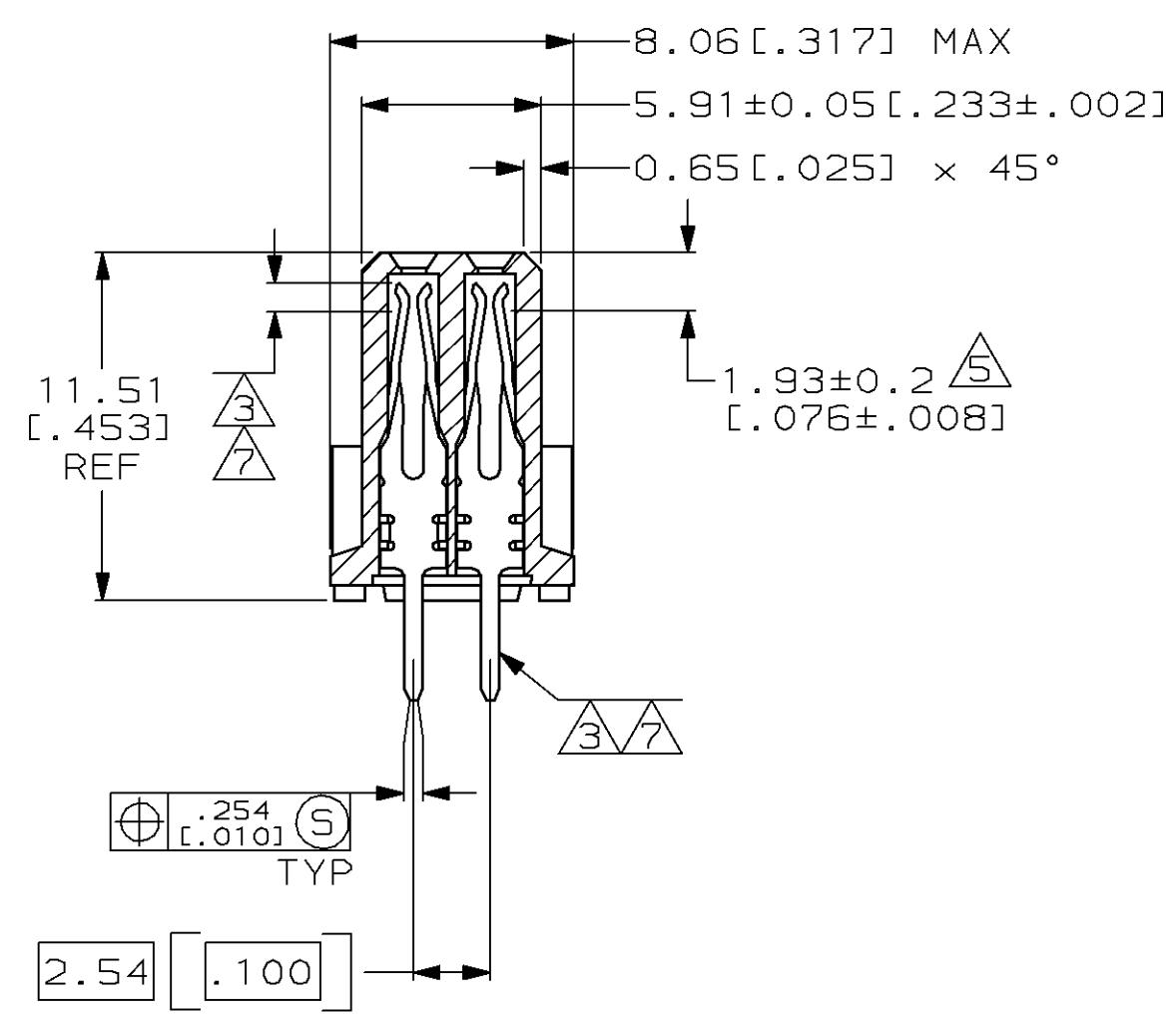
SECTION X-X
