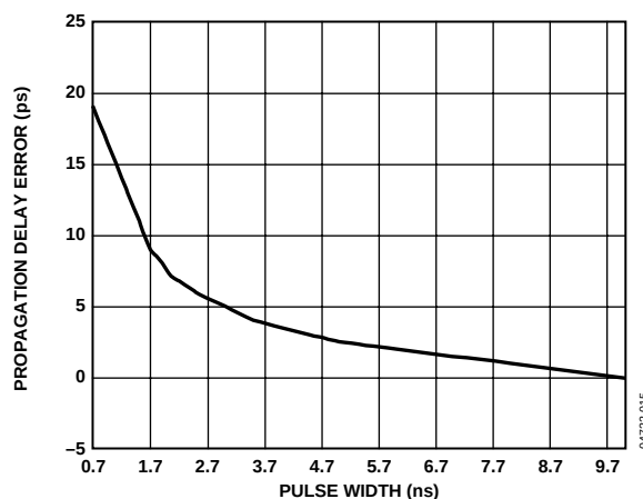
Figure 15. Propagation Delay Error vs. Pulse Width
