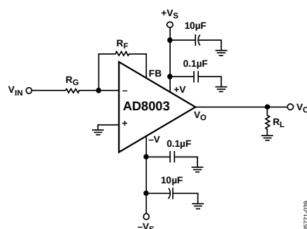
Figure 39. Inverting Gain
