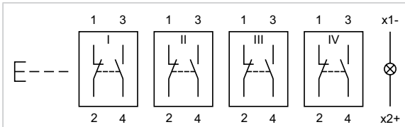
Wiring diagram 22
