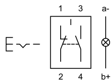
Wiring diagram 25
