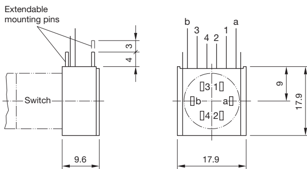
Component layout 1
