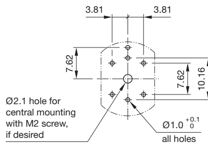
Component layout 2
