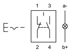
Wiring diagram 25
