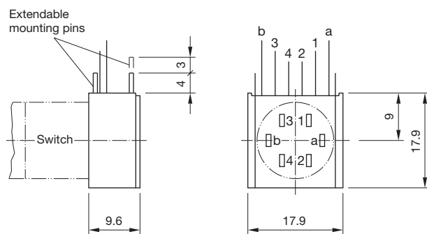
Component layout 1
