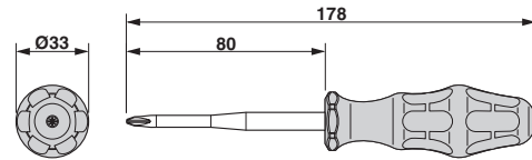
Dimensioned drawing
