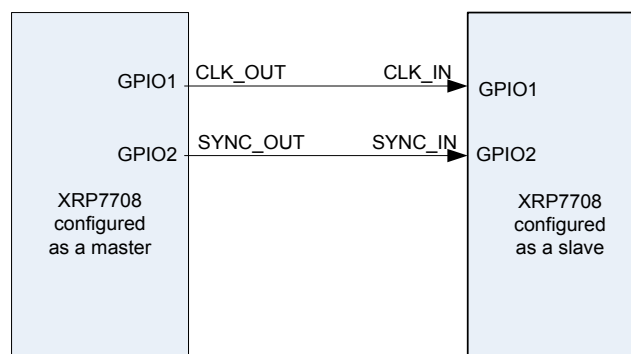
Fig. 23: Master/Slave Configuration of the XRP7708
