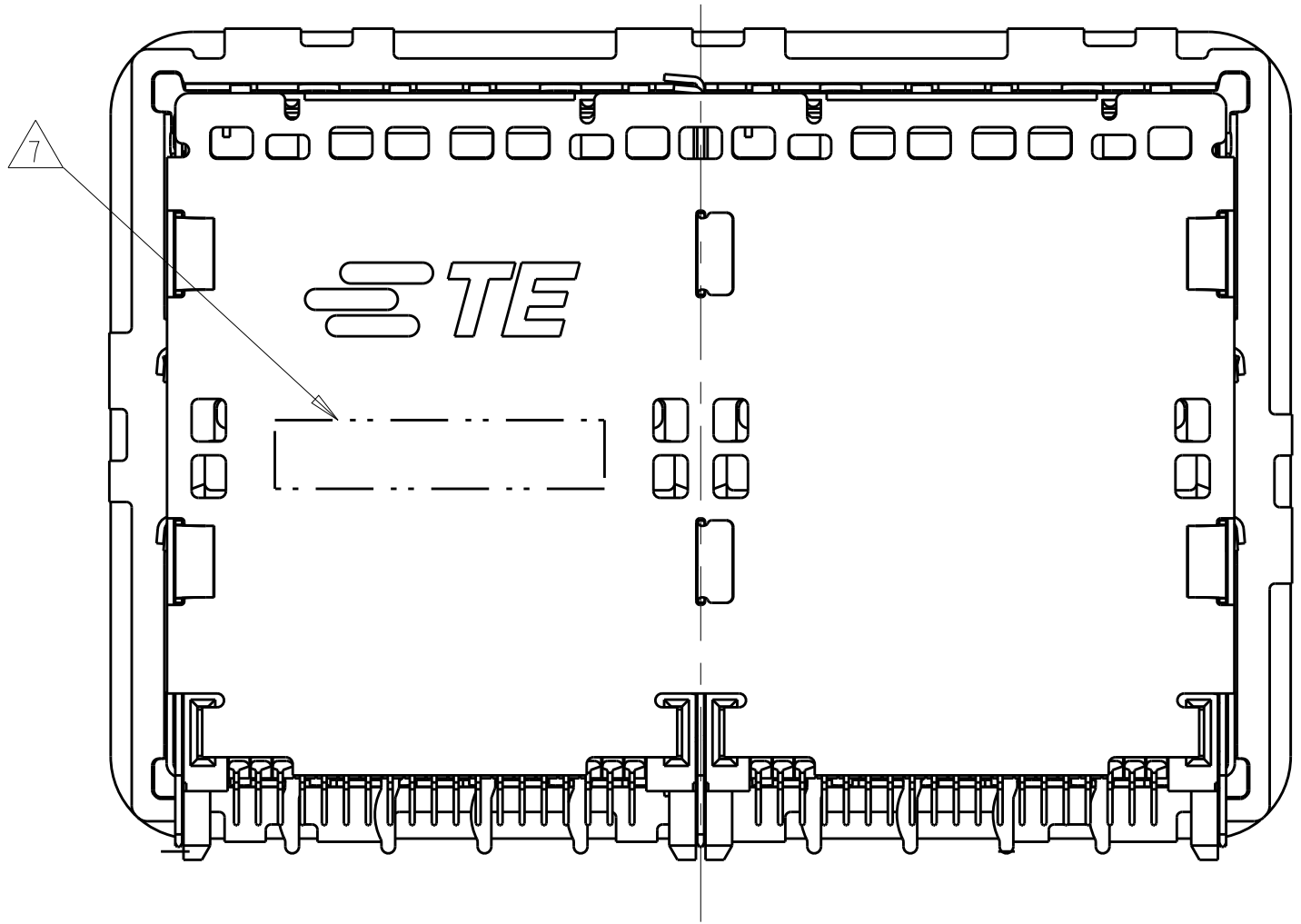
VIEW Y-Y
