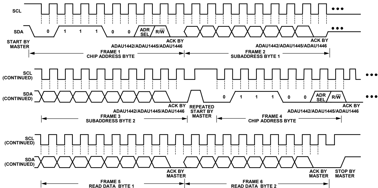
Figure 14. I²C Read Clocking
